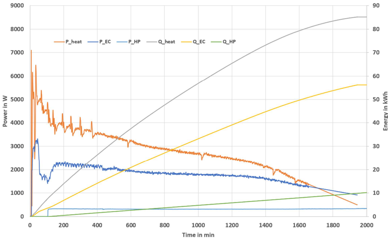
Figure 15 : Discharging of one main storage @ 35 °C
