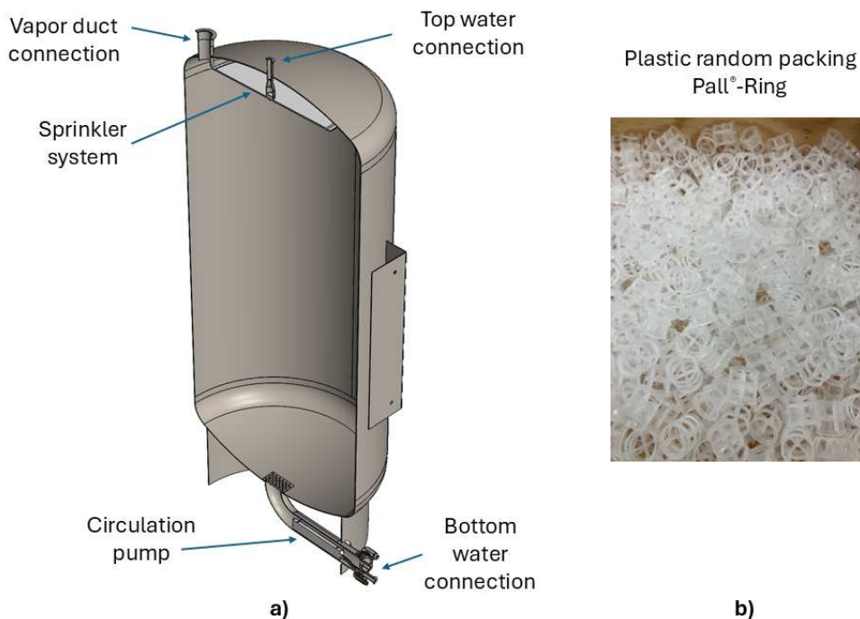
Figure 6 : Evaporator/condenser; a) section cut © Pink GmbH, b) random packing © AEE INTEC – A. Krainer
