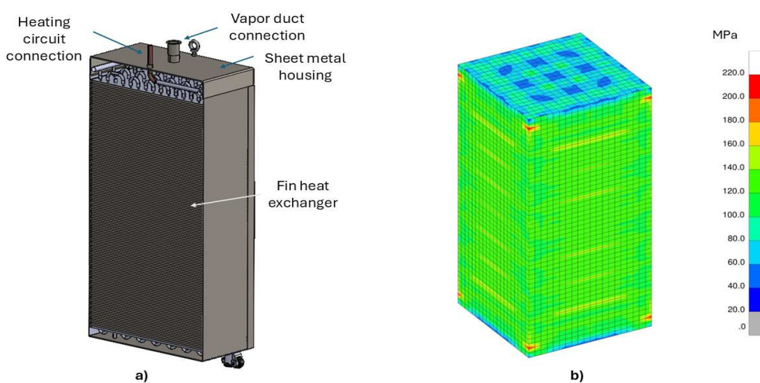
Figure 7 : Main sorption storage module; a) section cut of module and heat exchanger © Pink GmbH, b) strength simulation © SinusPro GmbH
