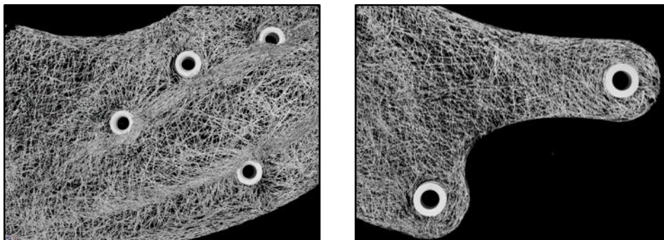
Figure 15: XCT scans of the transmission cross beam with glass fibre tracers.
