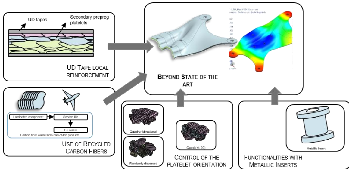
Figure 4: 0-WASTE concept to reduce carbon fibre waste in the production of structural lightweight automotive components.
