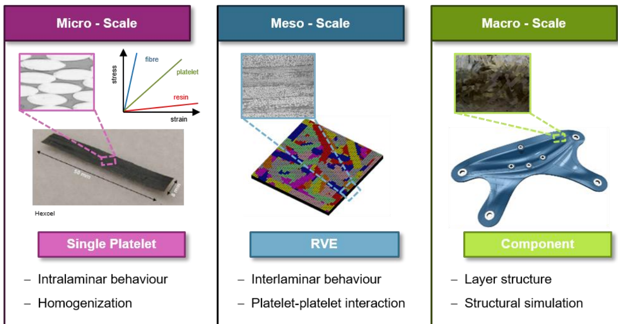
Figure 6: Multiscale simulation approach for the simulation of the SMC material behaviour.
