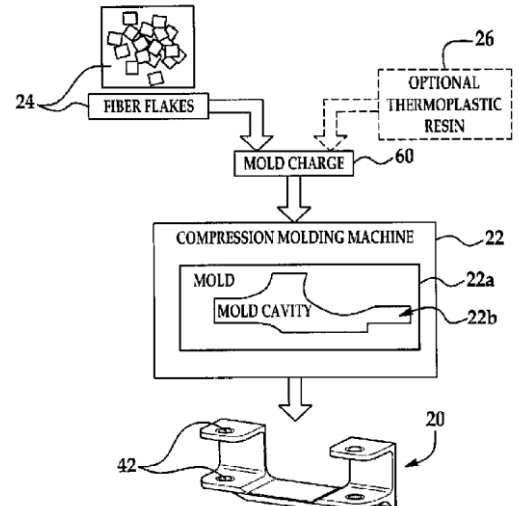
Figure 2: Compression moulding method for fibre reinforced thermoplastics (US8709319).
