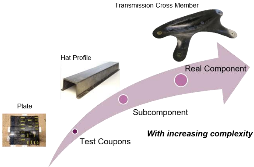
Figure 8: Increasing complexity of material characterisation.
