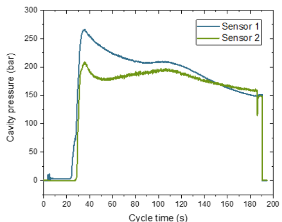
Figure 12: Optimized process parameters and the measured cavity pressure during the manufacture of the transmission cross beam.
