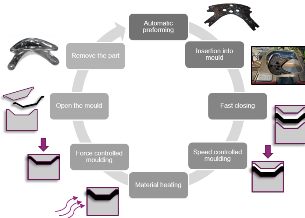
Figure 11: C-SMC compression moulding process.
