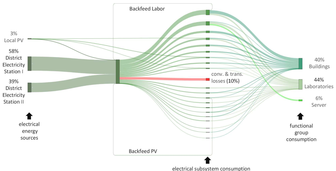
Figure 32: Illustration of electricity demand per functional group, in the Innovation District Inffeld (06.2022 – 06.2023)
