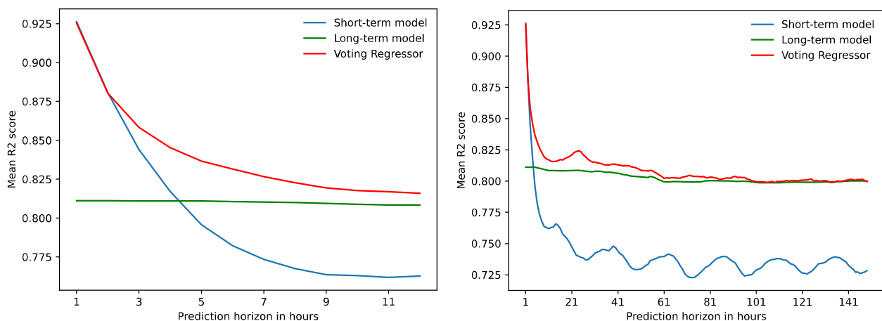
Figure 22: left: Comparison of the best performing short- and long-term models (both Random Forests), right: R2 scores from cross-validation of the Voting Regressor, short- and long-term models over a prediction horizon of 150 hours.
