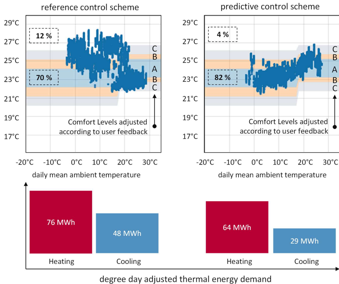
Figure 38: Zone air temperature of the first floor for the reference control scheme (top left) with the predictive control scheme (top right) in the reference timespan of one year. Comparison of heating and cooling energy (bottom).
