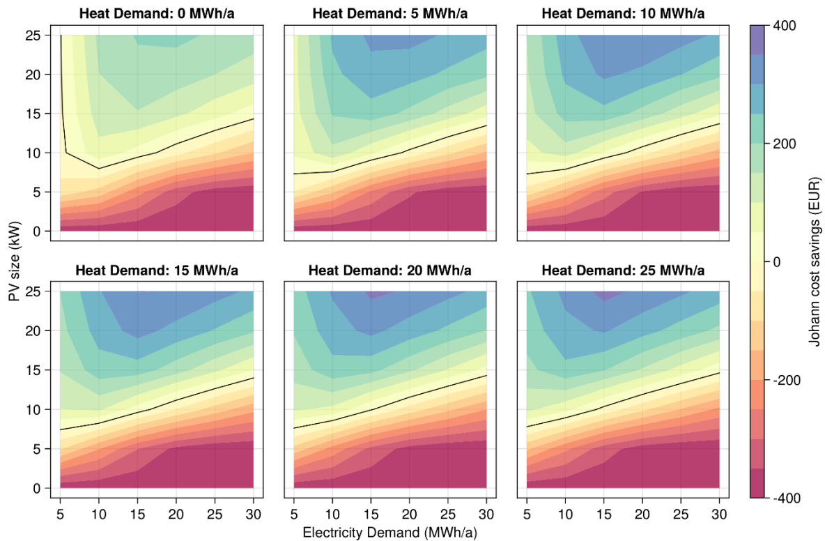
Figure 16: annual savings achieved with JOHANN for different combinations of heat demand, electricity demand and PV size.
