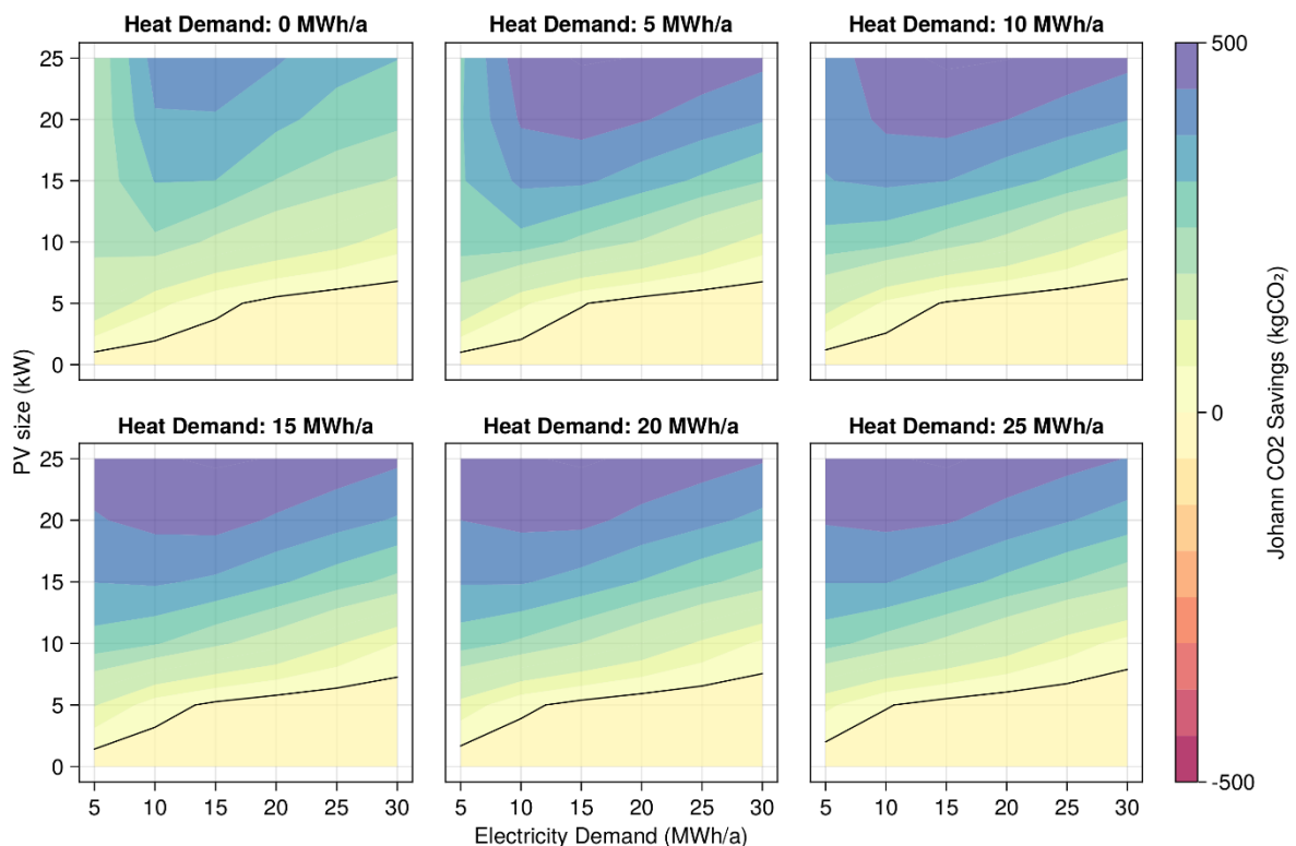
Figure 17: annual reductions in CO2 emissions achieved with JOHANN for different combinations of heat demand, electricity demand and PV size.
