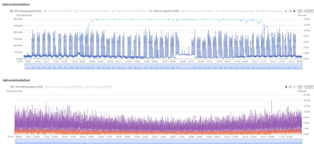
Figure 12: Results of a simulation (H2-storage, power consumption and heat delivery of a heatpump system) Johann control unit
